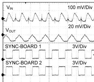
Figure 52. Output voltage ripple of two modules with synchronization clocks 180 degrees out of phase
