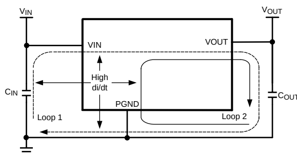
Figure 49. High Current Loops
