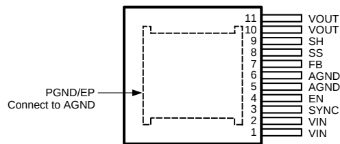
Figure 2. Top View - 11-Lead PFM
