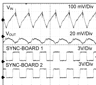
Figure 52. Output voltage ripple of two modules with synchronization clocks 180 degrees out of phase
