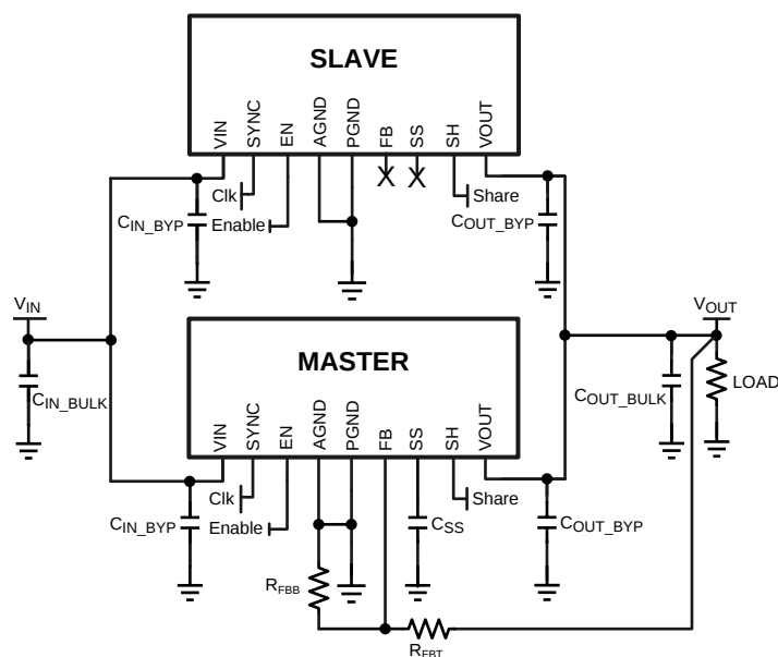
Figure 50. Current Sharing Example Schematic
