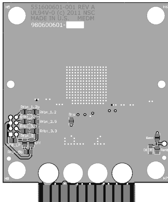
Figure 56. Layout example
